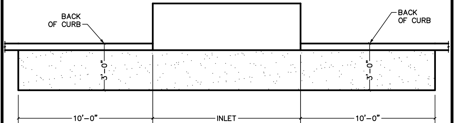
PAVEMENT BLOCKOUT
