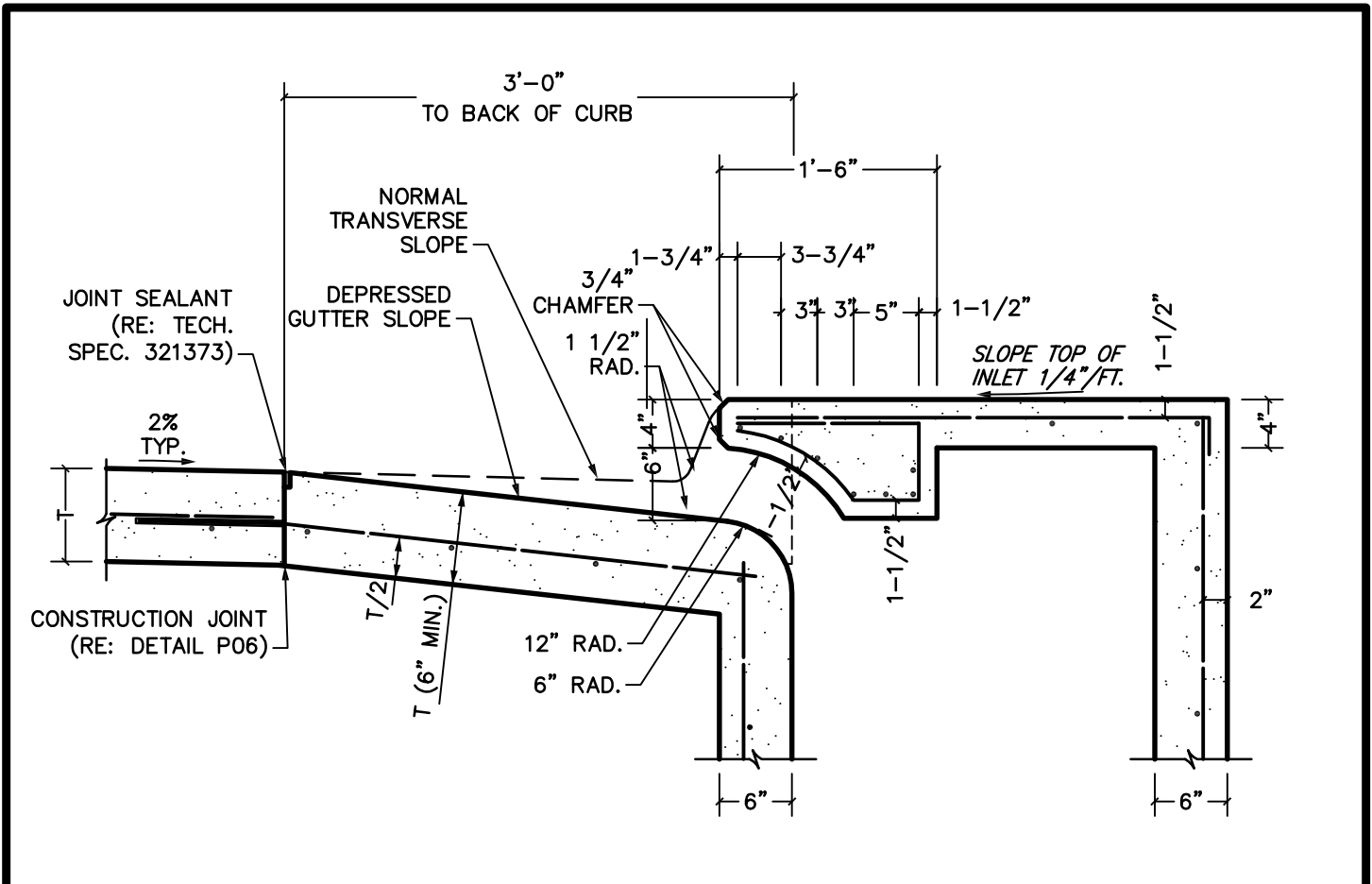
THROAT SECTION
